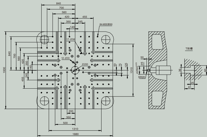
● UN1400A2
