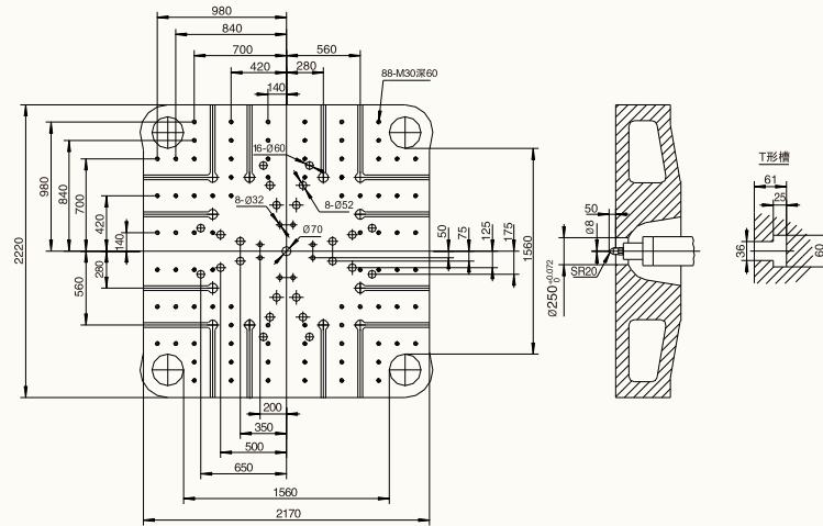
● UN1800A2
