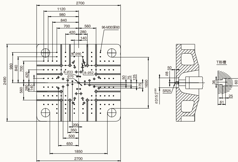
● UN2200A2
